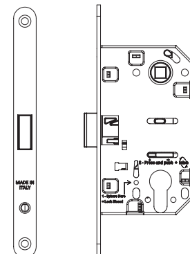
Foro cilindro Cylinder hole
