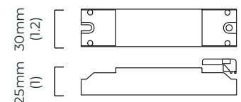
DALI converter dimensions
